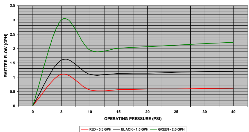
EMITTER DISCHARGE RATES AT VARIOUS OPERATING PRESSURES
