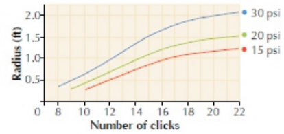
Radius of Throw 180°
